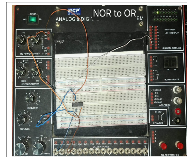
NOR to OR
